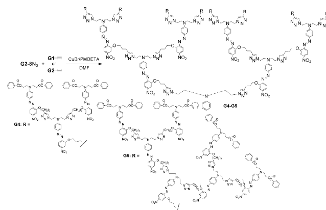
Scheme 2. Synthesis of dendrimers G4 and G5 .
