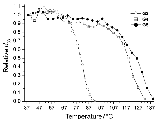
Figure 1. Decay curves for the SHG coefficient d_{33} of G3–G5 as a function of temperature.
