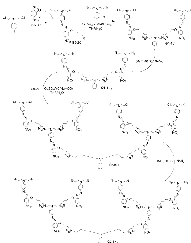
Scheme 1. Synthesis of the core ( G2–8N 3 ) of the dendrimers.
